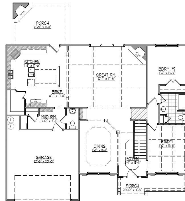
"The Cedar" FIRST FLOORPLAN
