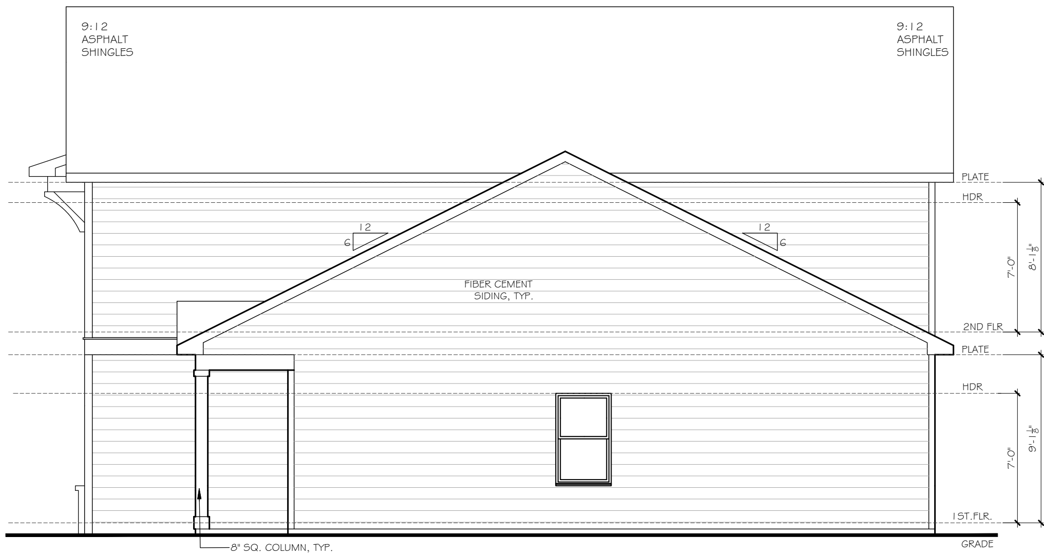
3 RIGHT ELEVATION SCALE: 3/16" = 1'-0"
