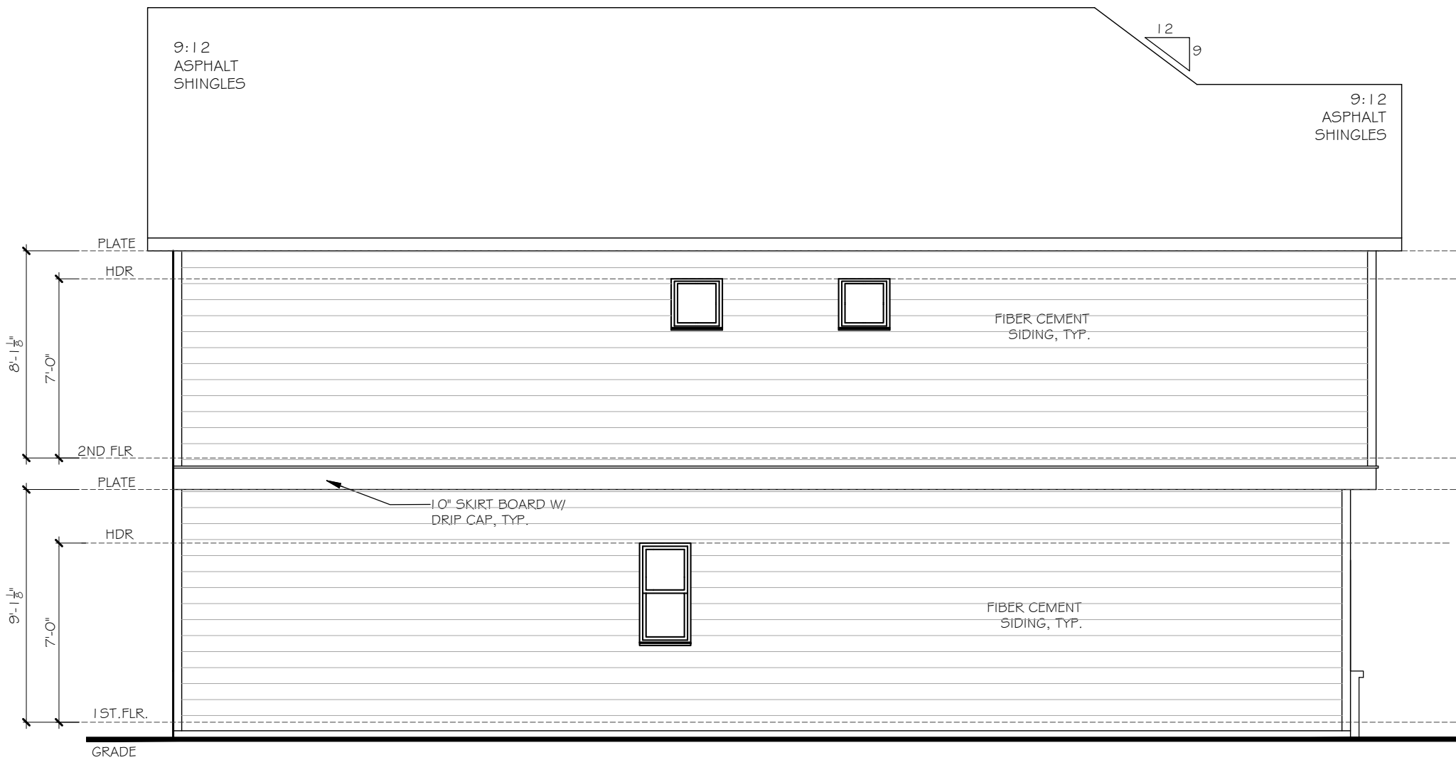
2 LEFT ELEVATION SCALE: 3/16" = 1'-0"
